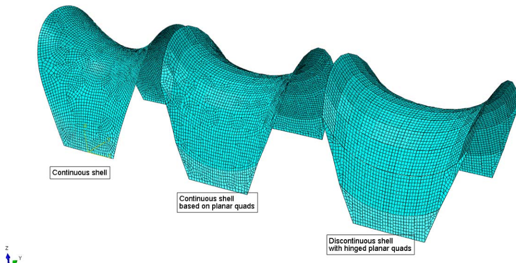
Figure 7: Model plot with mesh of the three models
